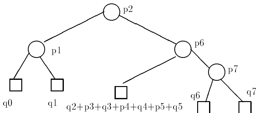
Figure 2: An example of a special subtree with respect to (l, r) = (2, 6) . The keys are in the circles and the intervals between the keys correspond to square nodes. The tree covers interval (1, 7) with the gap between keys numbered l = 2, r = 6 .
