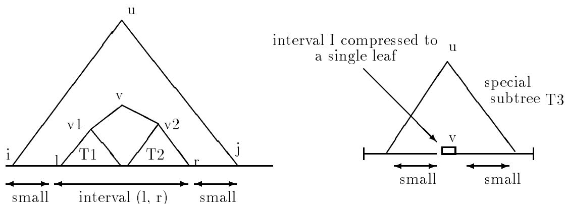
Figure 3: A decomposition of the subtree in \Gamma_{k+1} . The subtrees T1, T2 rooted at v1, v2 are in \Gamma_1 \cup \Gamma_2 \cup \dots \cup \Gamma_k . A special tree T3 results by replacing the interval I by a single leaf whose weight equals the total weight w(l, r) of I .
