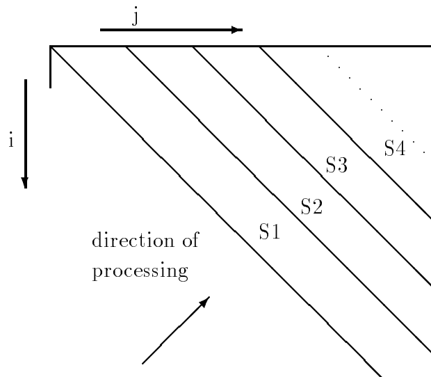
Figure 1: The dynamic programming table and its partition into the strips.
